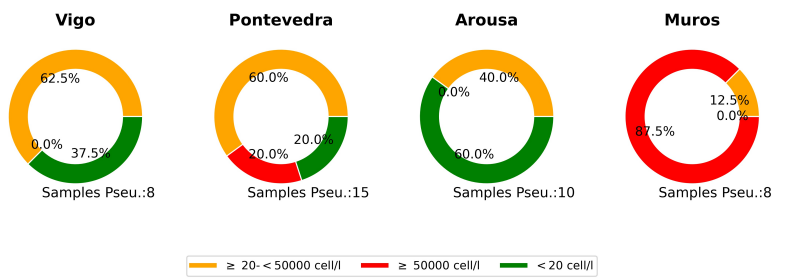
Pseudo-nitzschia spp.
